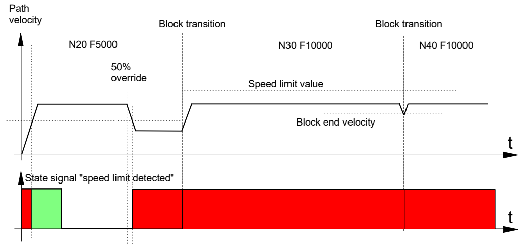
Fig. 4: Timing diagram without override weighting ( f\_override\_weight\_v\_limit = 0 )
