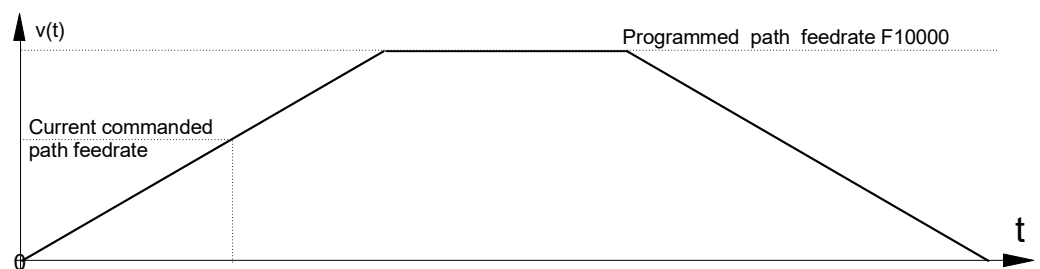
Fig. 2: Path velocity at D_ActiveFeed
