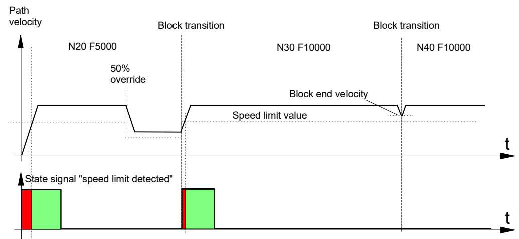
Fig. 5: Timing diagram with override weighting ( f\_override\_weight\_v\_limit = 1 )
