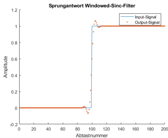
Abb. 7: Sprungantwort Windowed-Sinc-Filter
