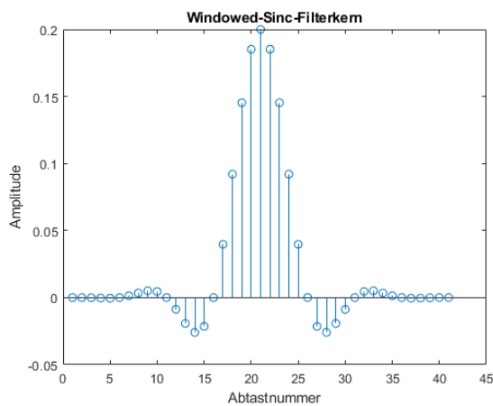
Abb. 6: Filterkern Windowed-Sinc-Filter
