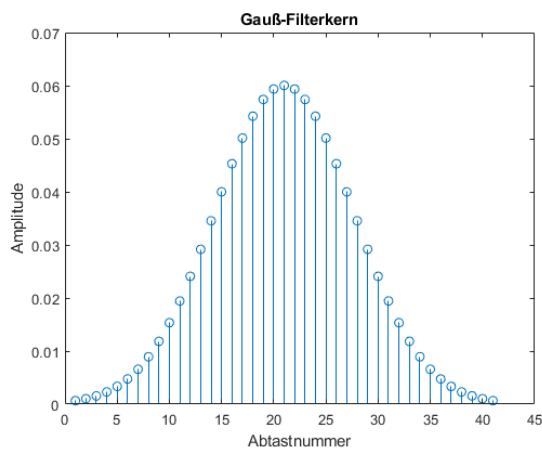
Abb. 4: Filterkern Gauß-Filter
